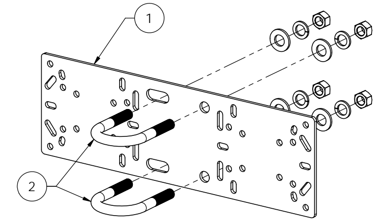
EXPLODED ISO VIEW
