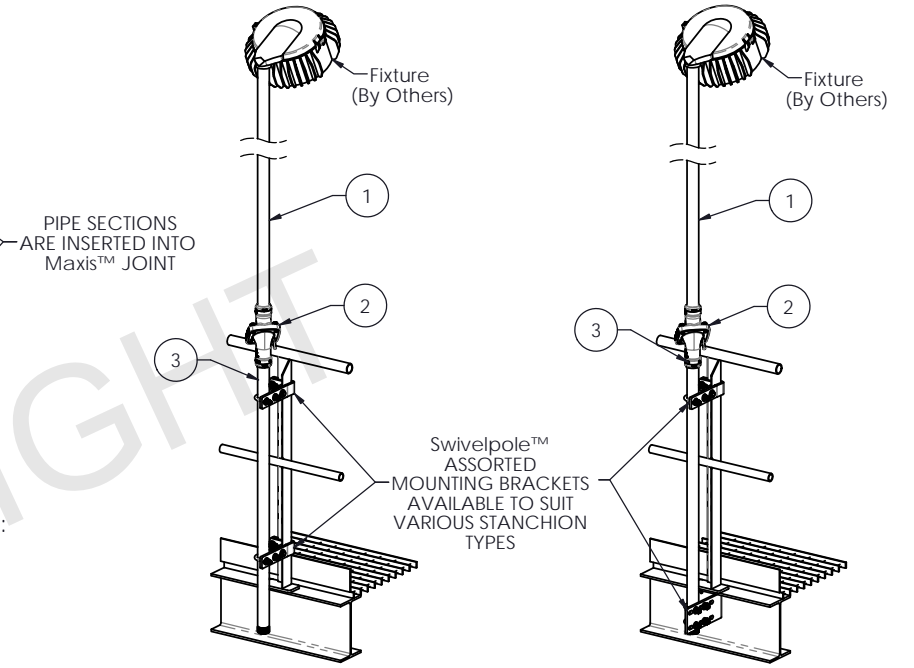
S3-M1 STANCHION MOUNTED ASSEMBLY VIEW
