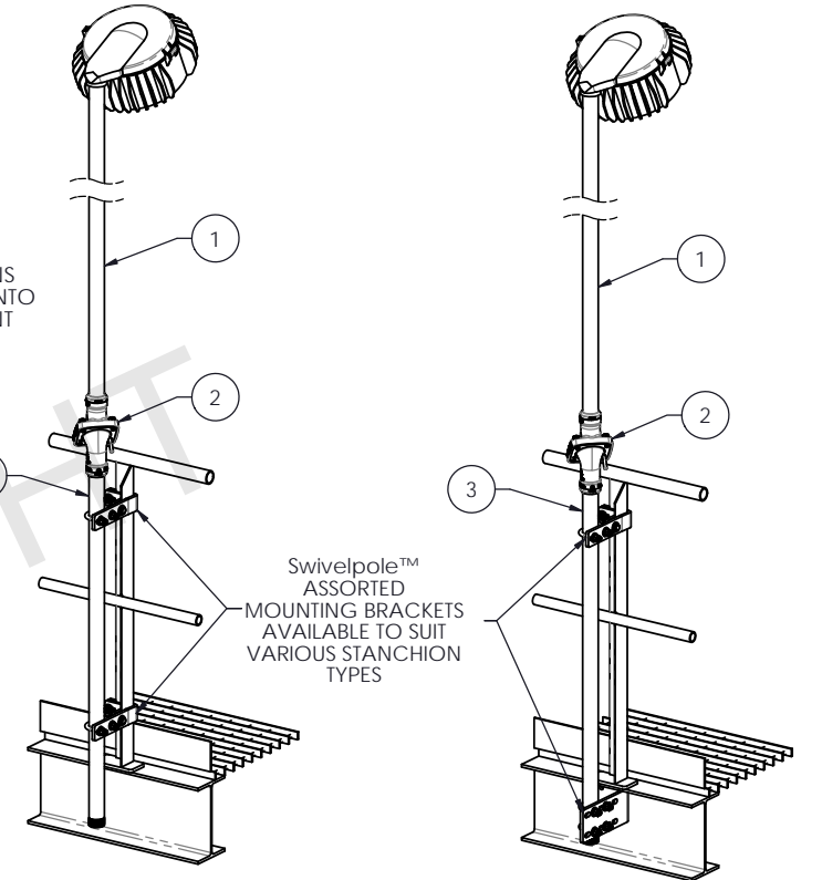
S3-M1 STANCHION MOUNTED ASSEMBLY VIEW
